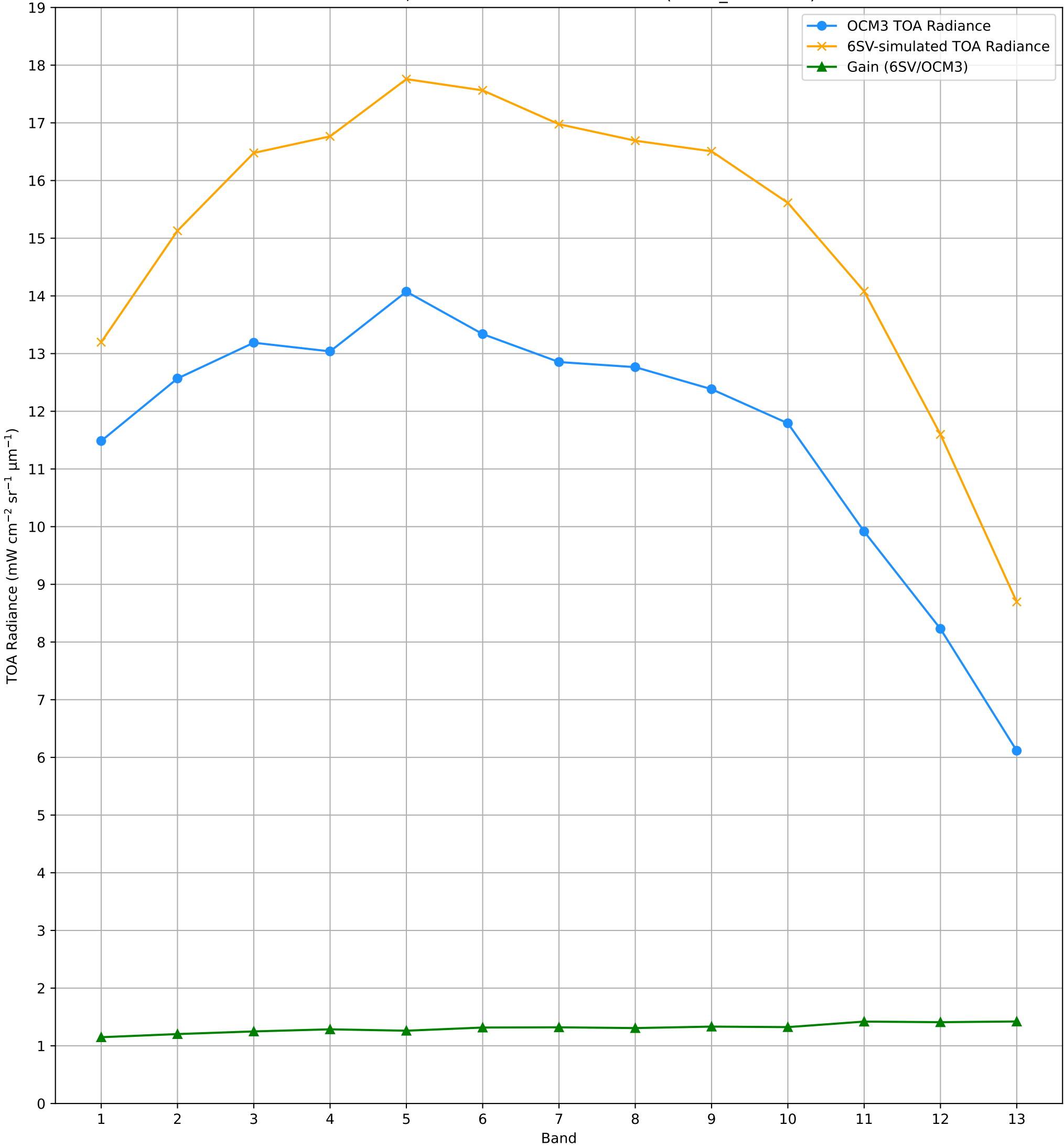
TOA Radiance (OCM3 vs. 6SV) over RVUS RadCalNet Site Lat: 38.497°, Lon: -115.69° - 16-AUG-2025 (STRIP_ID: 14384)
