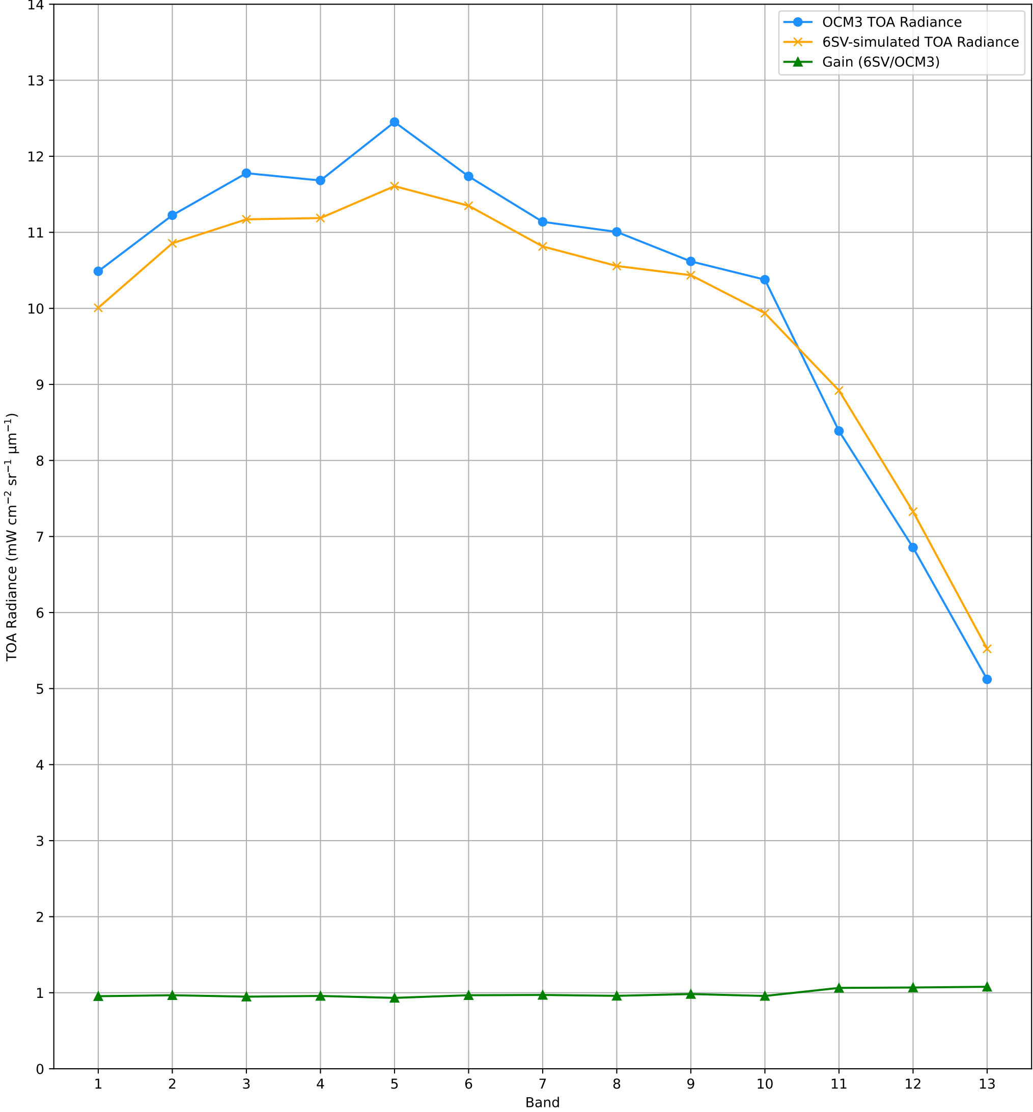
TOA Radiance (OCM3 vs. 6SV) over RVUS RadCalNet Site Lat: 38.497°, Lon: -115.69° - 03-NOV-2025 (STRIP_ID: 15526)
