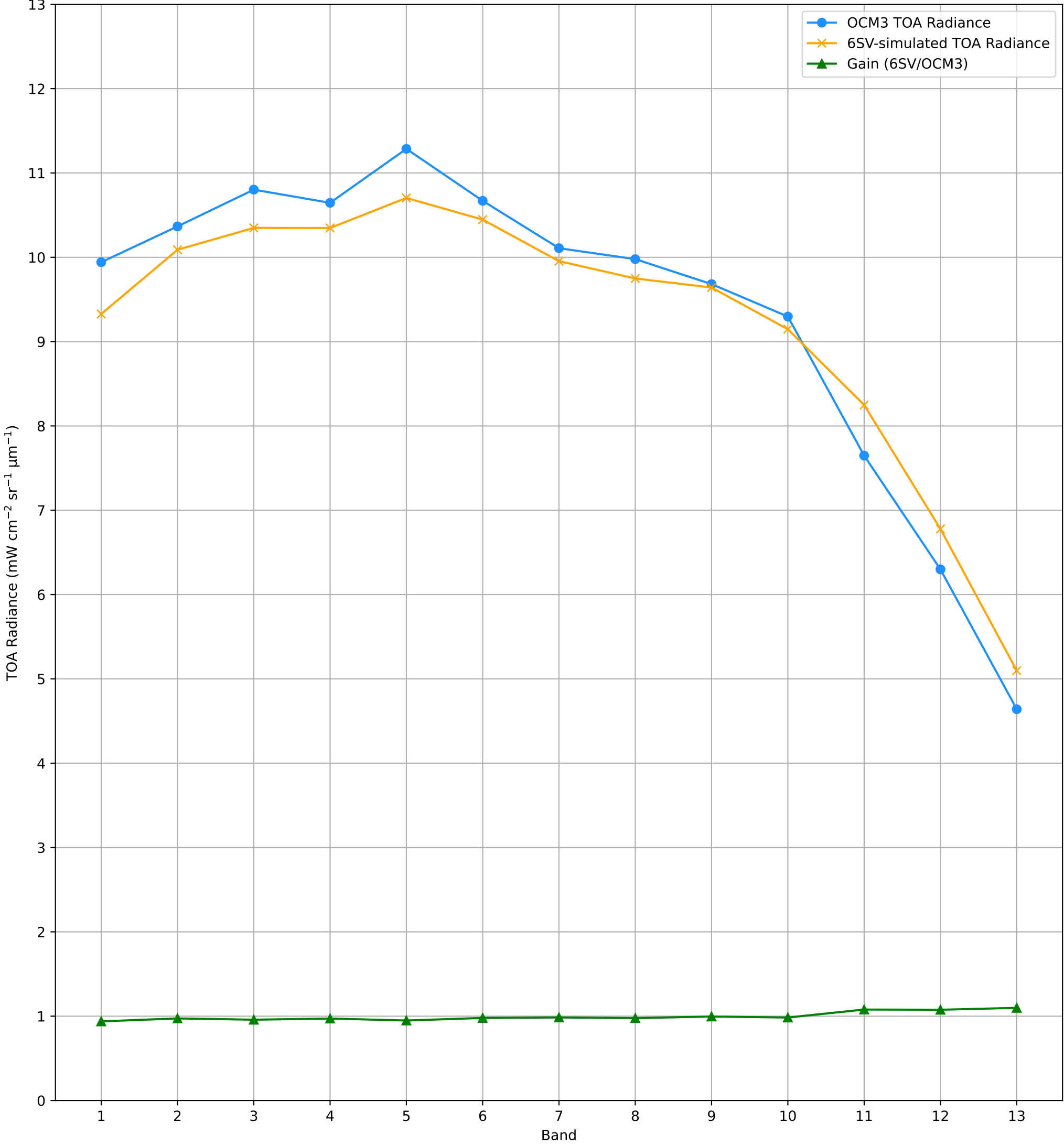
TOA Radiance (OCM3 vs. 6SV) over RVUS RadCalNet Site Lat: 38.497°, Lon: -115.69° - 09-NOV-2025 (STRIP_ID: 15613)
