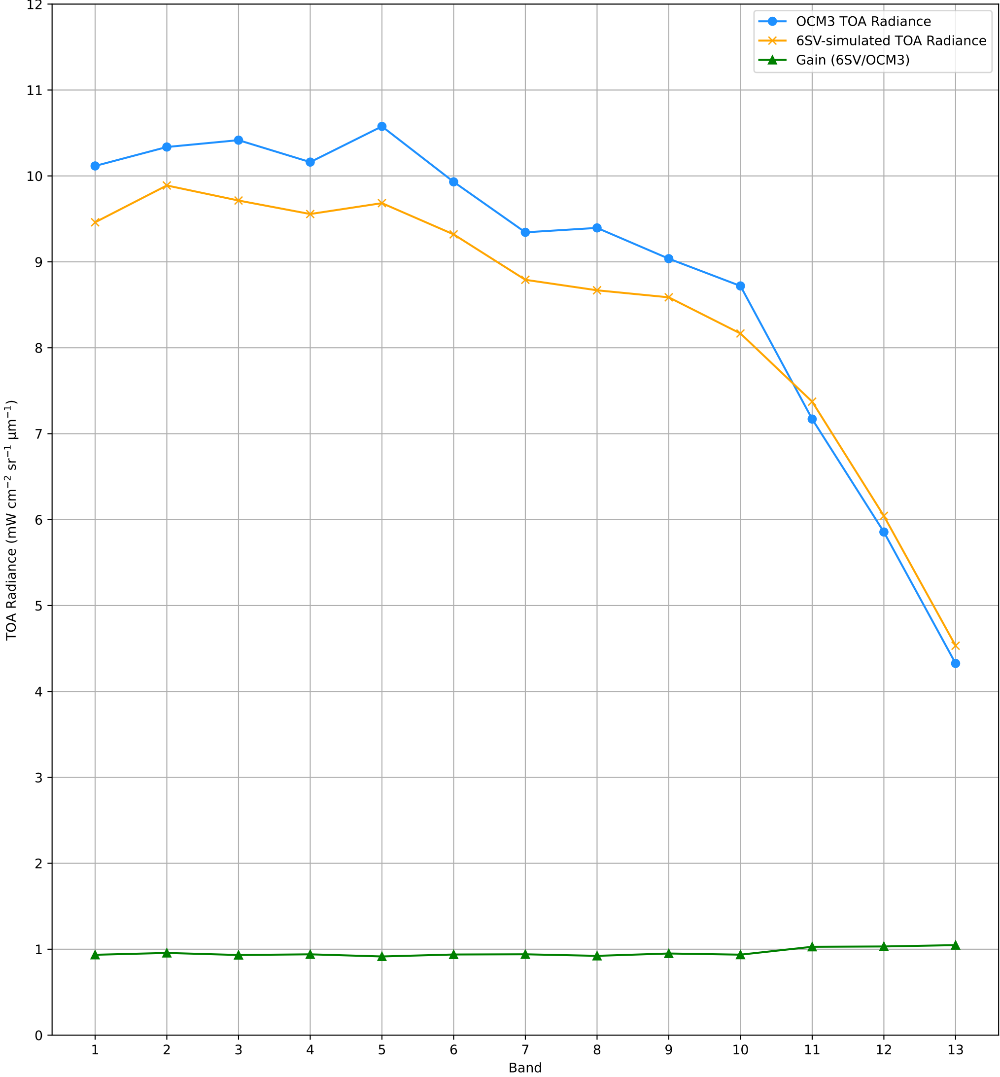
TOA Radiance (OCM3 vs. 6SV) over RVUS RadCalNet Site Lat: 38.497°, Lon: -115.69° - 23-NOV-2025 (STRIP_ID: 15815)
