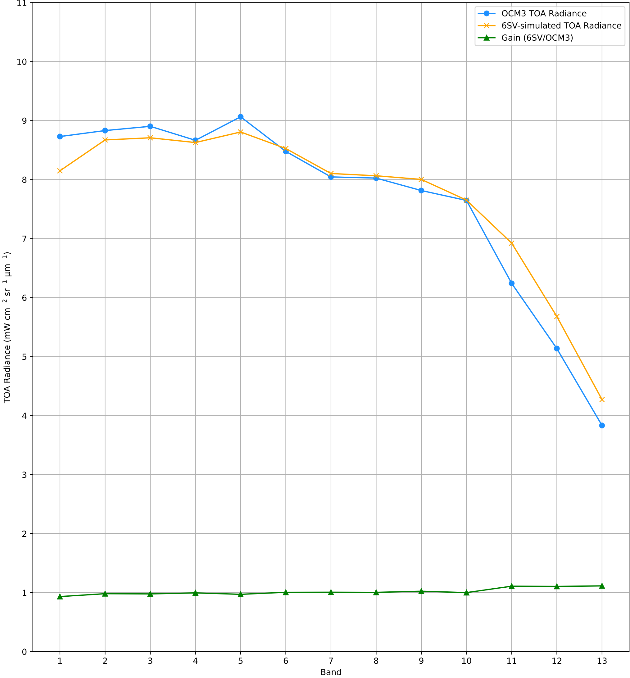
TOA Radiance (OCM3 vs. 6SV) over RVUS RadCalNet Site Lat: 38.497°, Lon: -115.69° - 24-NOV-2025 (STRIP_ID: 15830)
