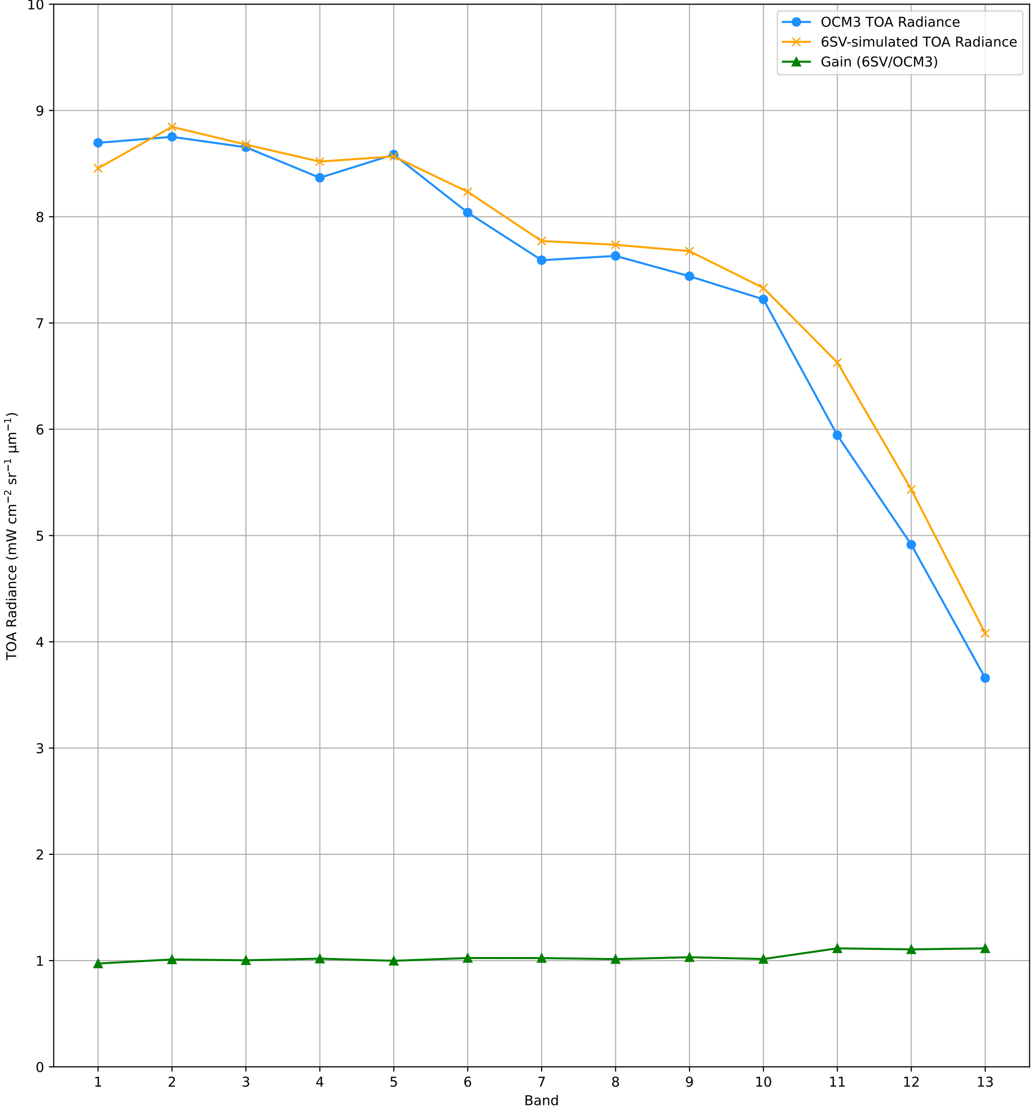
TOA Radiance (OCM3 vs. 6SV) over RVUS RadCalNet Site Lat: 38.497°, Lon: -115.69° - 28-NOV-2025 (STRIP_ID: 15888)
