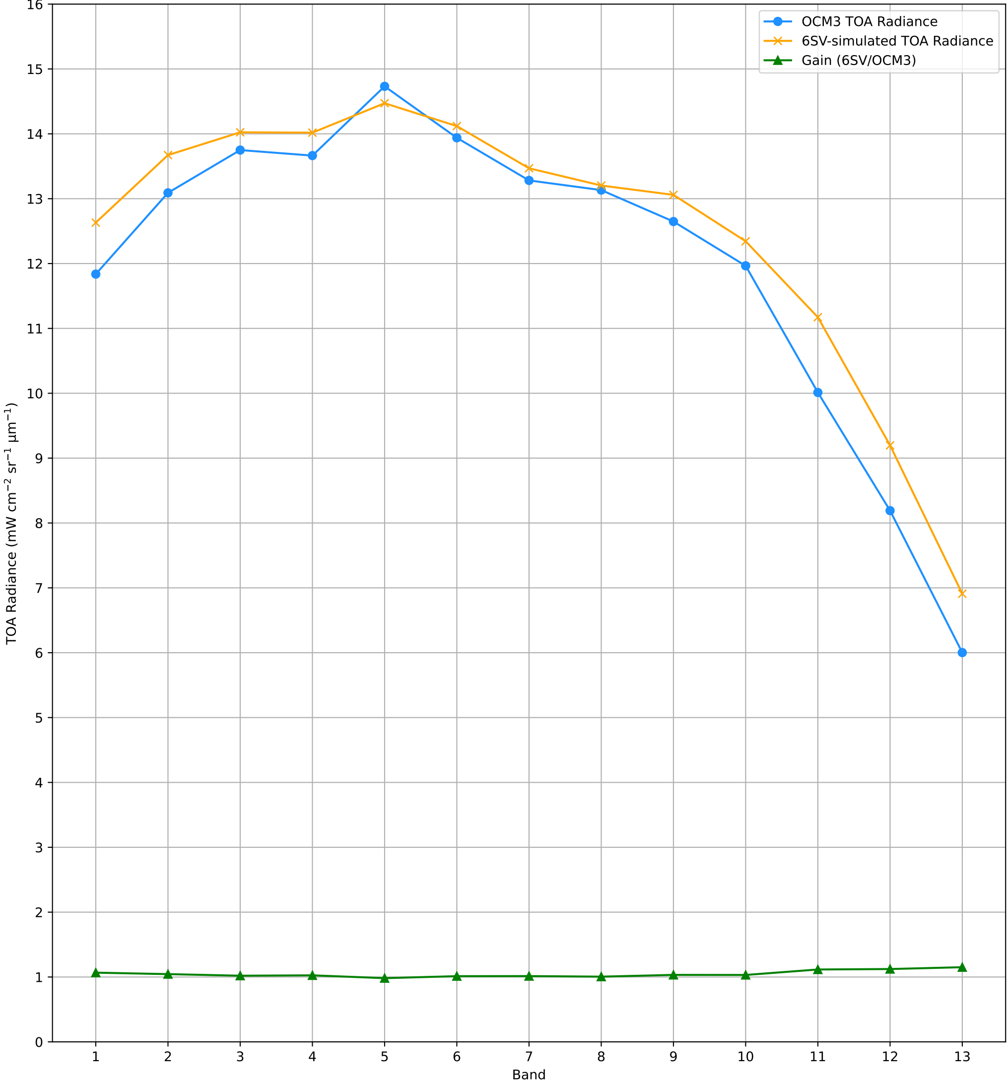
TOA Radiance (OCM3 vs. 6SV) over RVUS RadCalNet Site Lat: 38.497°, Lon: -115.69° - 02-OCT-2025 (STRIP_ID: 15063)
