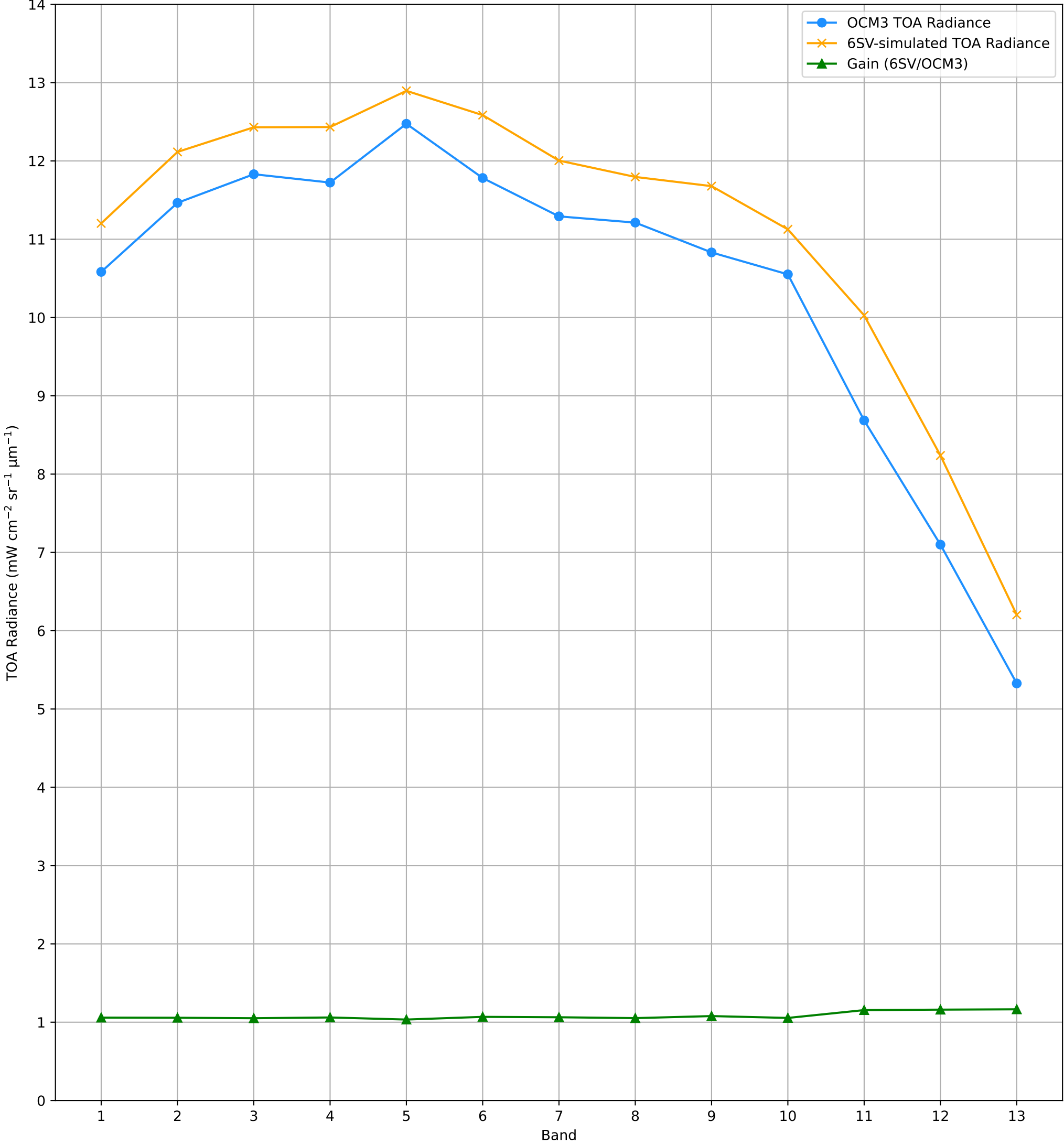
TOA Radiance (OCM3 vs. 6SV) over RVUS RadCalNet Site Lat: 38.497°, Lon: -115.69° - 05-OCT-2025 (STRIP_ID: 15107)
