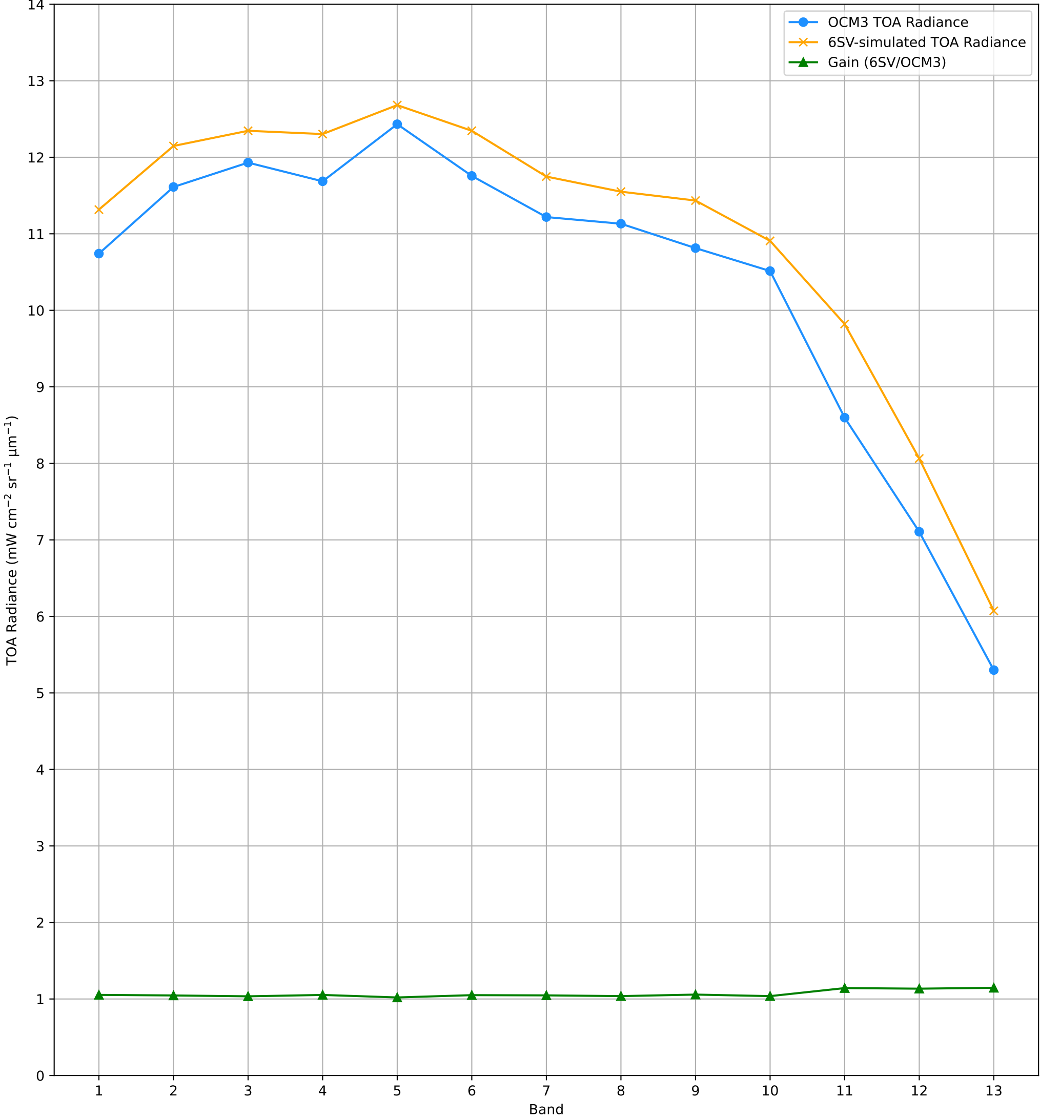
TOA Radiance (OCM3 vs. 6SV) over RVUS RadCalNet Site Lat: 38.497°, Lon: -115.69° - 07-OCT-2025 (STRIP_ID: 15136)
