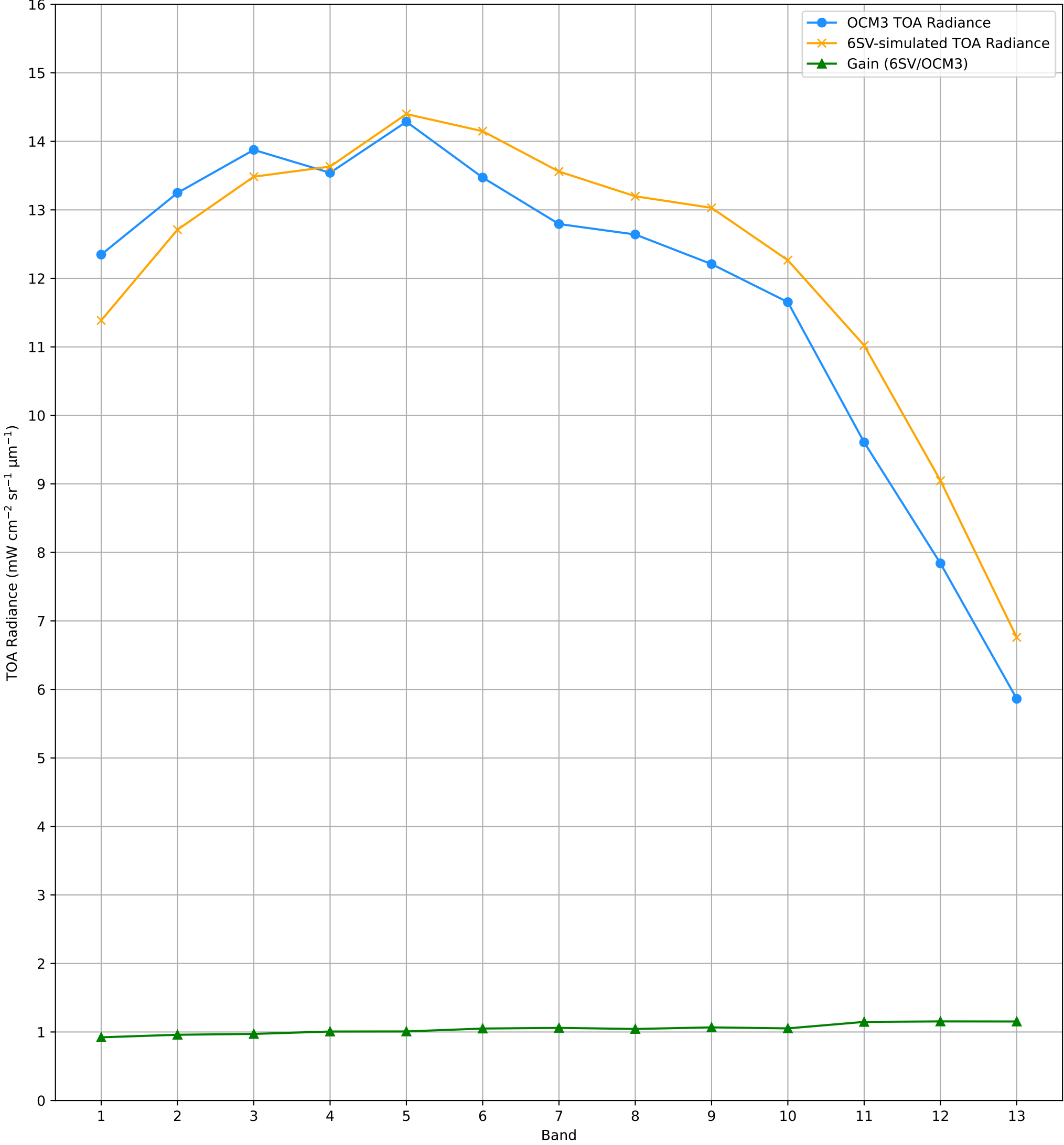
TOA Radiance (OCM3 vs. 6SV) over RVUS RadCalNet Site Lat: 38.497°, Lon: -115.69° - 10-OCT-2025 (STRIP_ID: 15179)
