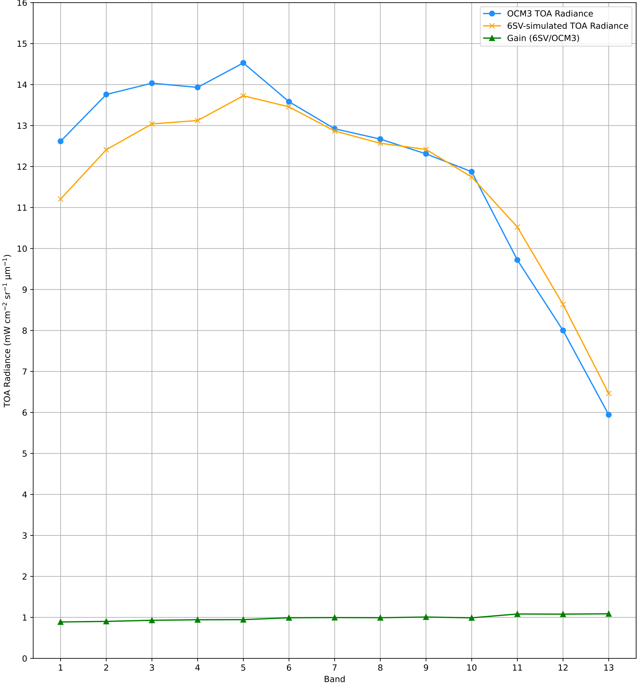
TOA Radiance (OCM3 vs. 6SV) over RVUS RadCalNet Site Lat: 38.497°, Lon: -115.69° - 16-OCT-2025 (STRIP_ID: 15266)
