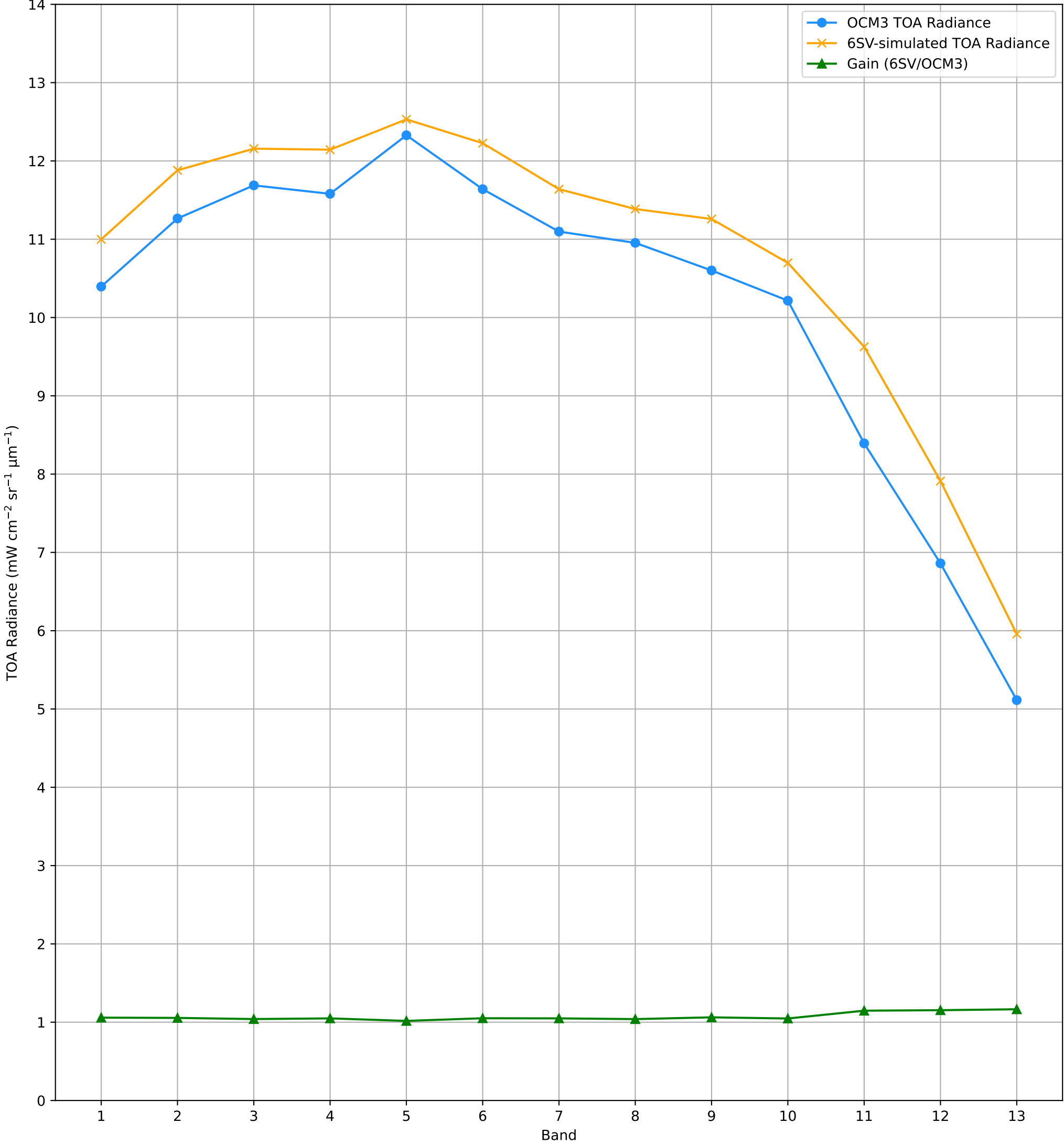
TOA Radiance (OCM3 vs. 6SV) over RVUS RadCalNet Site Lat: 38.497°, Lon: -115.69° - 18-OCT-2025 (STRIP_ID: 15295)
