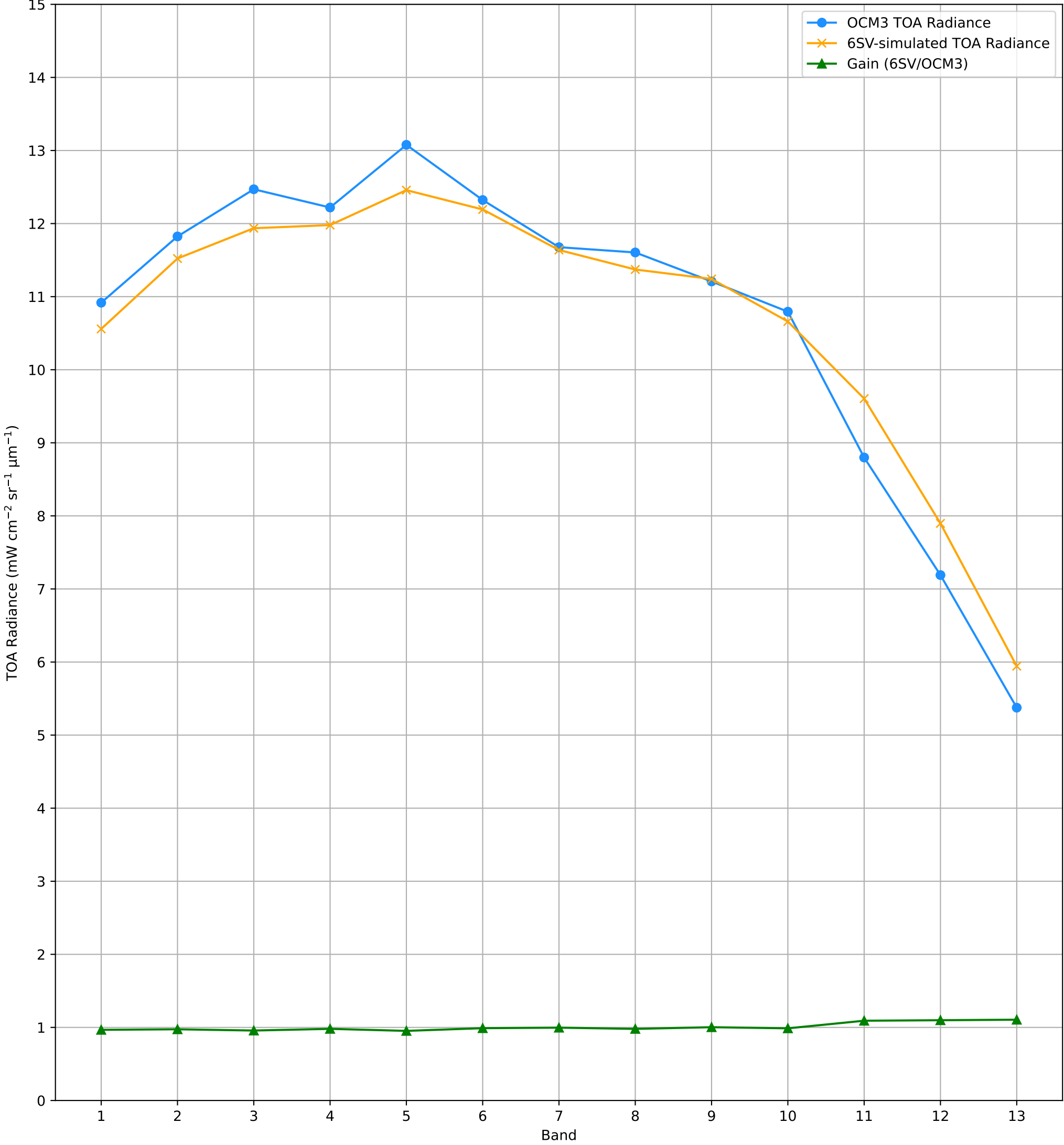
TOA Radiance (OCM3 vs. 6SV) over RVUS RadCalNet Site Lat: 38.497°, Lon: -115.69° - 23-OCT-2025 (STRIP_ID: 15367)
