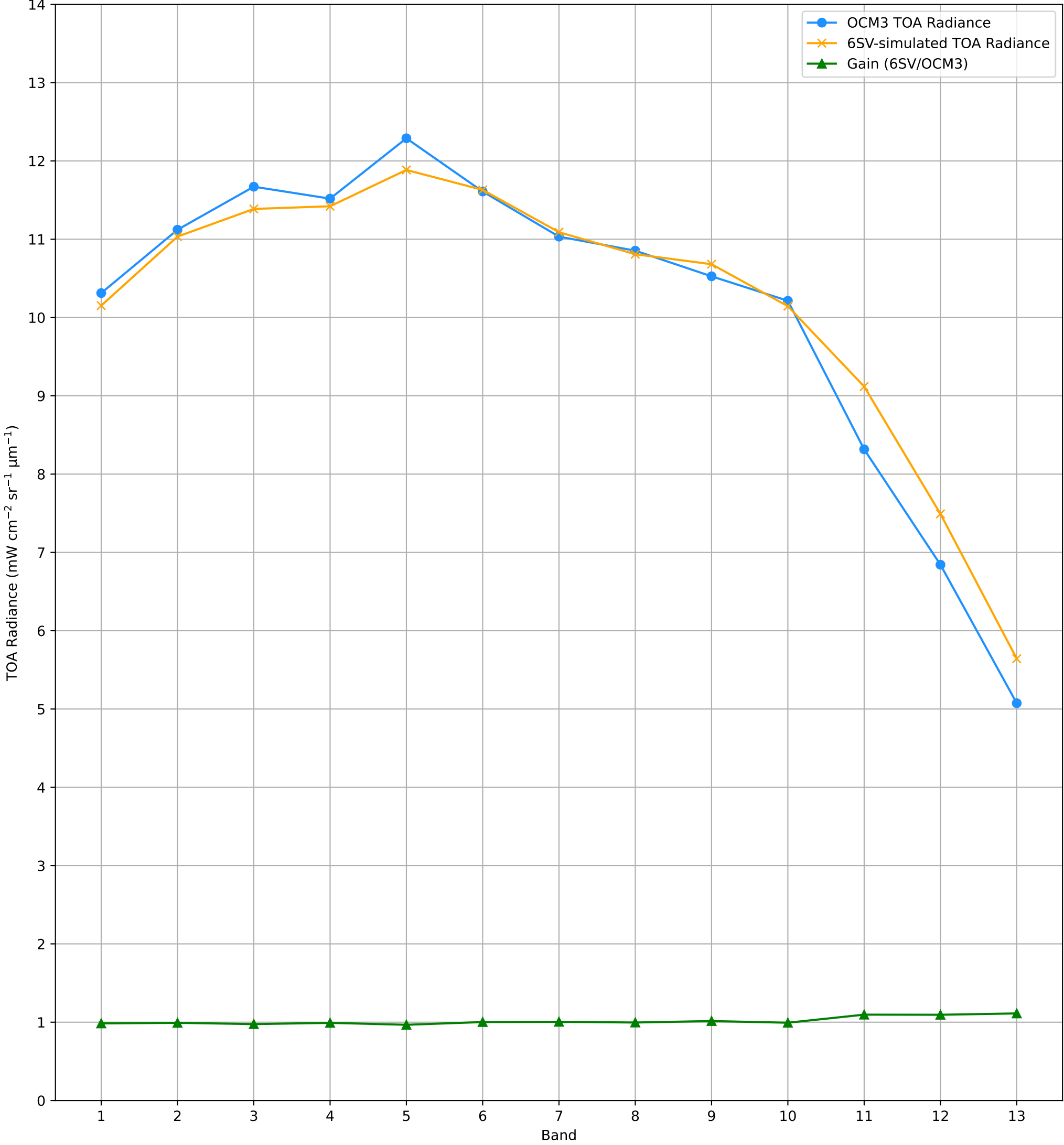
TOA Radiance (OCM3 vs. 6SV) over RVUS RadCalNet Site Lat: 38.497°, Lon: -115.69° - 27-OCT-2025 (STRIP_ID: 15425)
