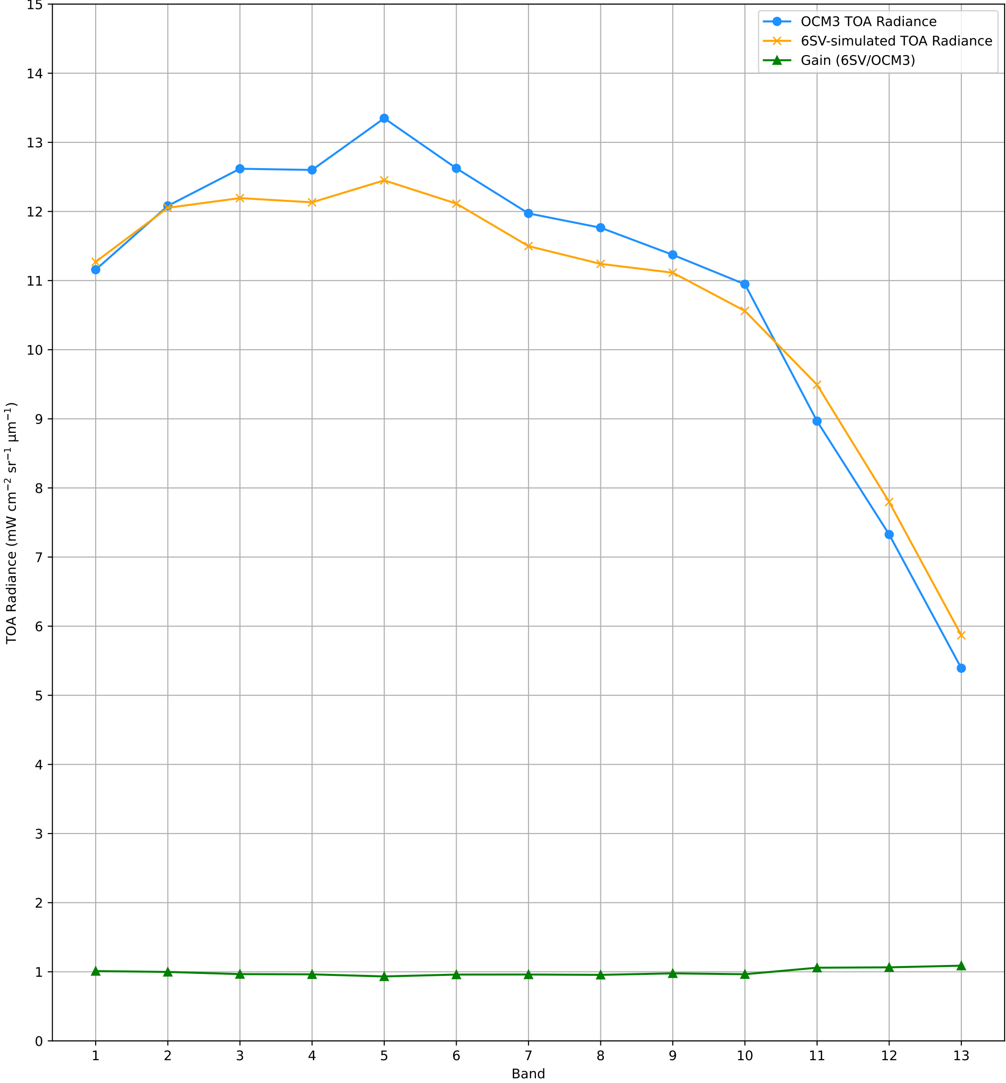
TOA Radiance (OCM3 vs. 6SV) over RVUS RadCalNet Site Lat: 38.497°, Lon: -115.69° - 28-OCT-2025 (STRIP_ID: 15439)
