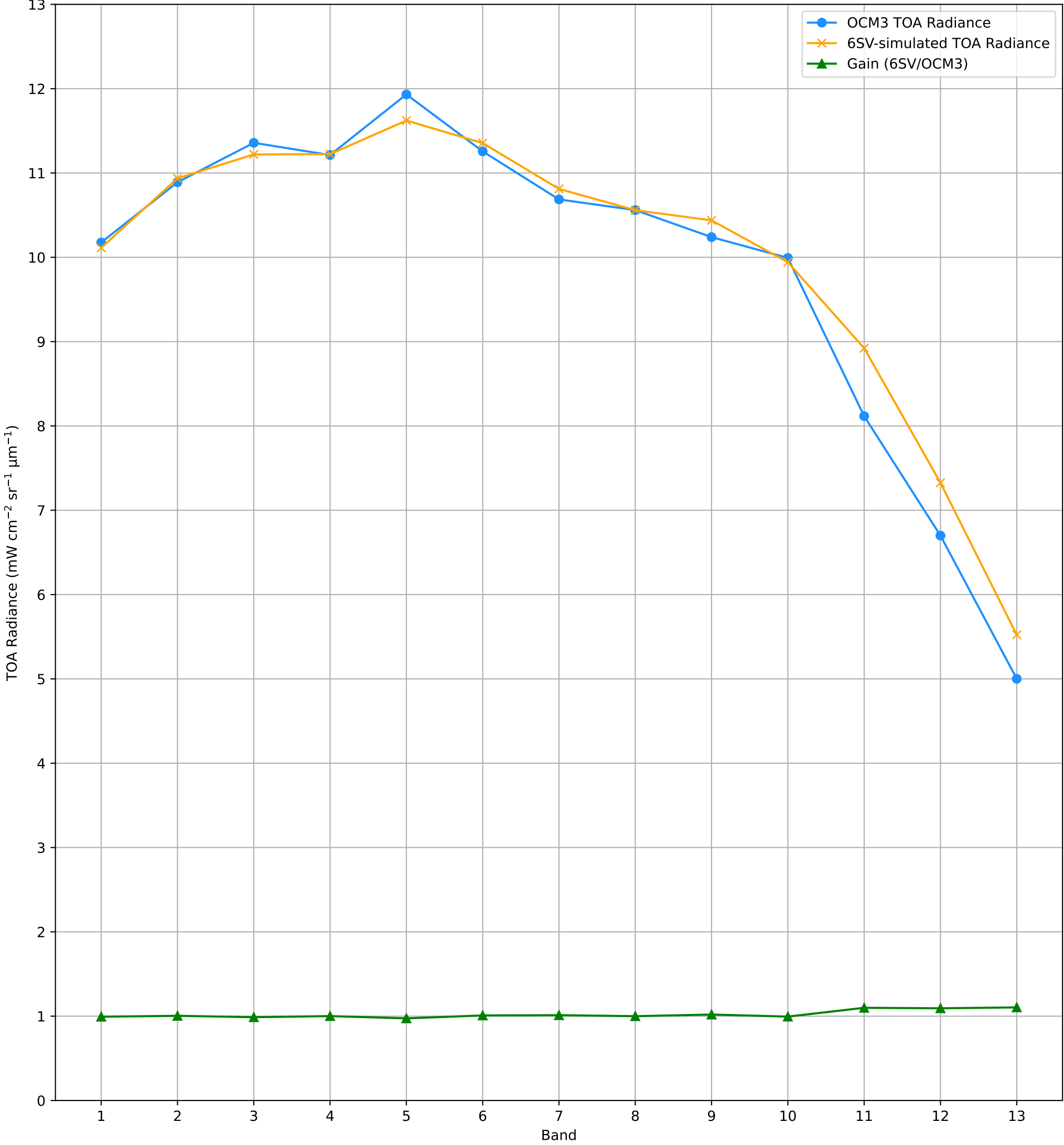
TOA Radiance (OCM3 vs. 6SV) over RVUS RadCalNet Site Lat: 38.497°, Lon: -115.69° - 29-OCT-2025 (STRIP_ID: 15454)
