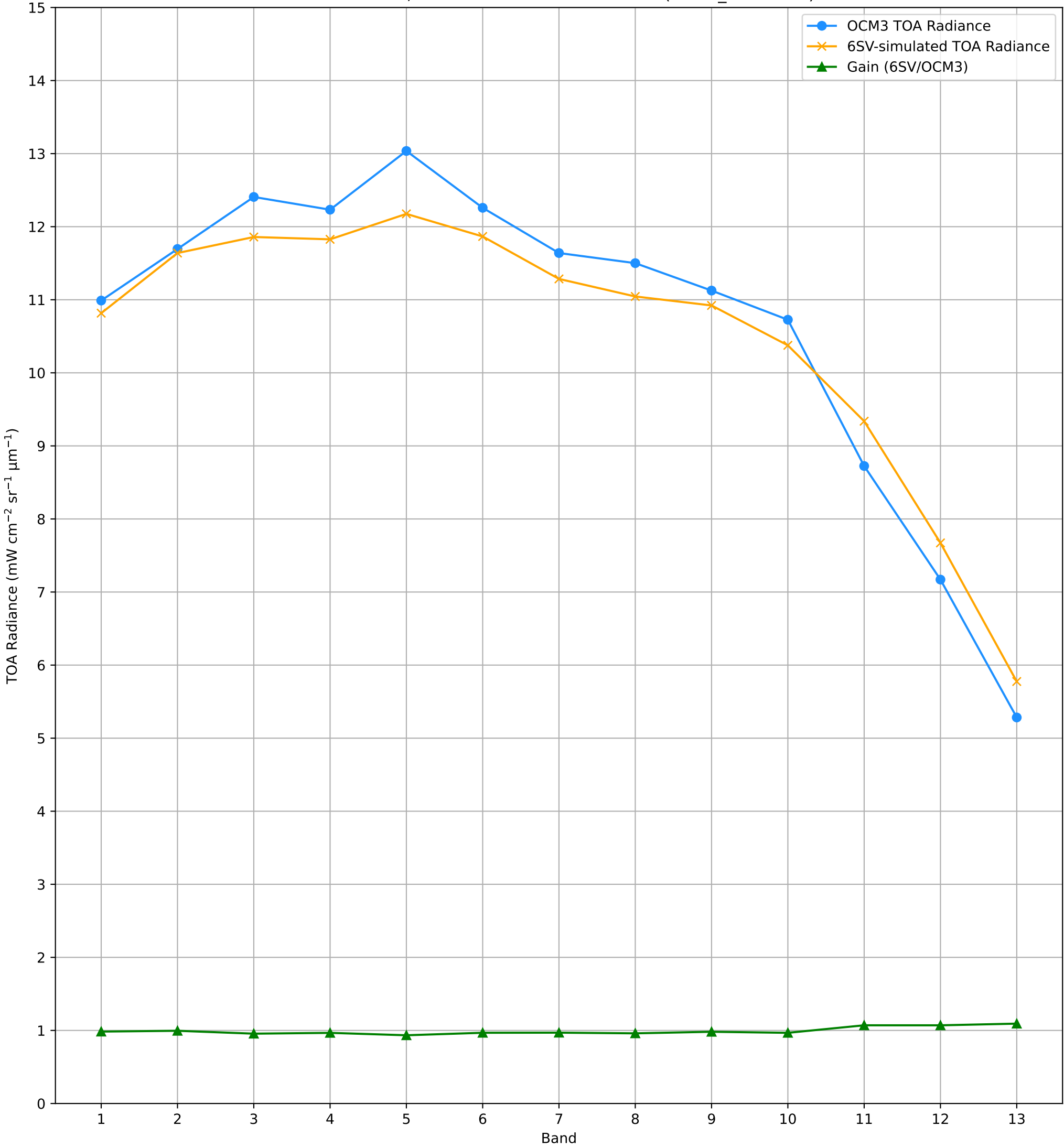
TOA Radiance (OCM3 vs. 6SV) over RVUS RadCalNet Site Lat: 38.497°, Lon: -115.69° - 30-OCT-2025 (STRIP_ID: 15468)
