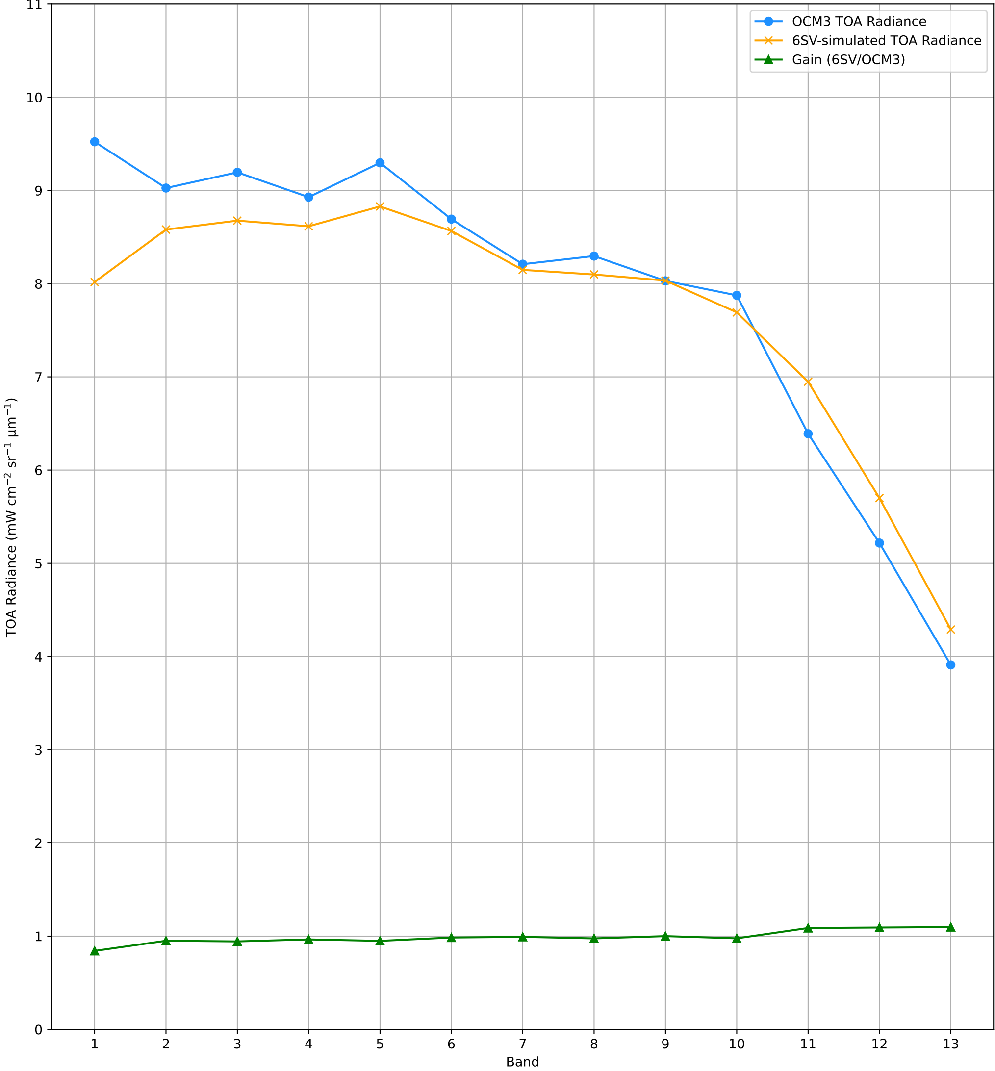
TOA Radiance (OCM3 vs. 6SV) over RVUS RadCalNet Site Lat: 38.497°, Lon: -115.69° - 01-DEC-2025 (STRIP_ID:15931)
