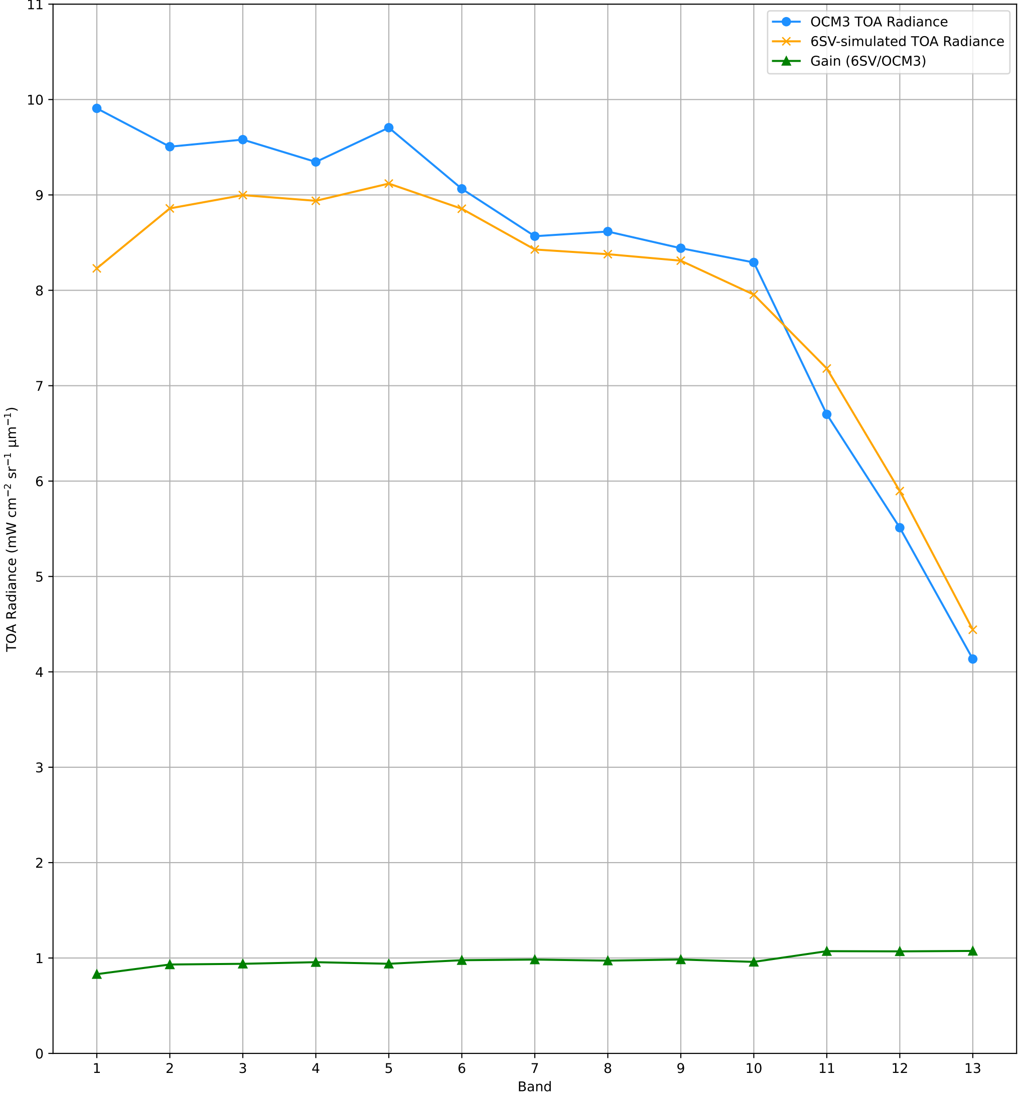
TOA Radiance (OCM3 vs. 6SV) over RVUS RadCalNet Site Lat: 38.497°, Lon: -115.69° - 03-DEC-2025 (STRIP_ID:15960)
