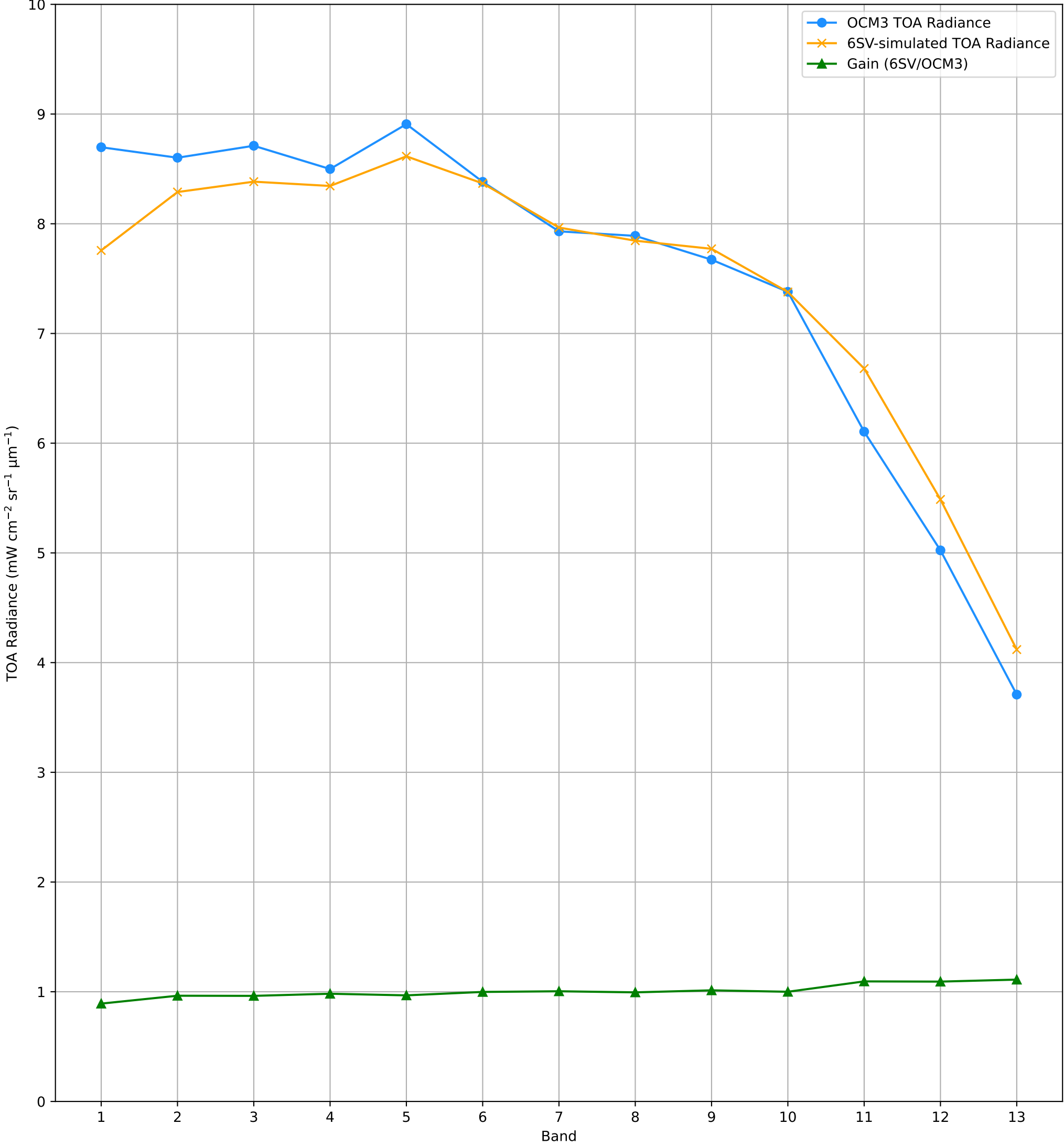
TOA Radiance (OCM3 vs. 6SV) over RVUS RadCalNet Site Lat: 38.497°, Lon: -115.69° - 05-DEC-2025 (STRIP_ID:15989)
