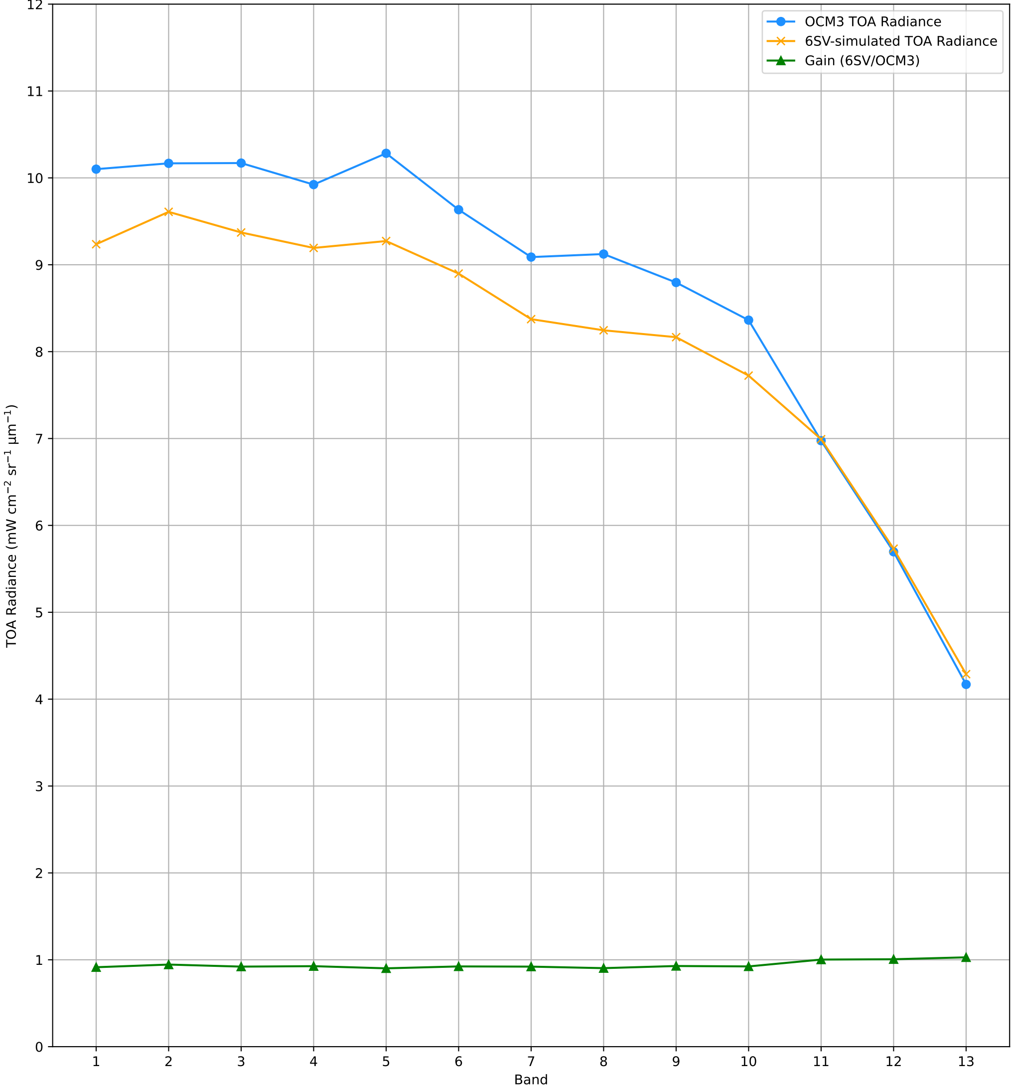
TOA Radiance (OCM3 vs. 6SV) over RVUS RadCalNet Site Lat: 38.497°, Lon: -115.69° - 06-DEC-2025 (STRIP_ID:16003)
