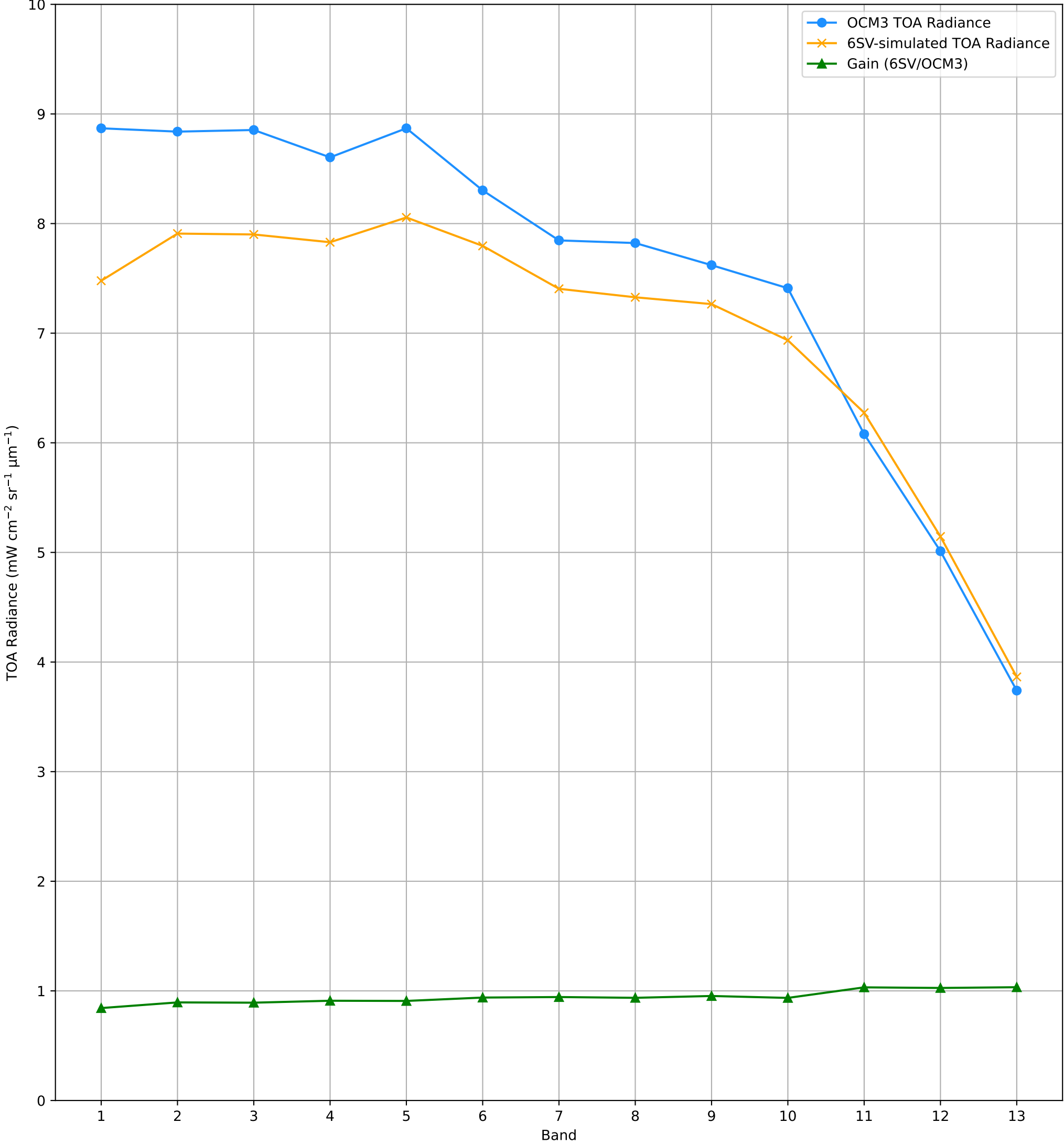
TOA Radiance (OCM3 vs. 6SV) over RVUS RadCalNet Site Lat: 38.497°, Lon: -115.69° - 07-DEC-2025 (STRIP_ID:16018)
