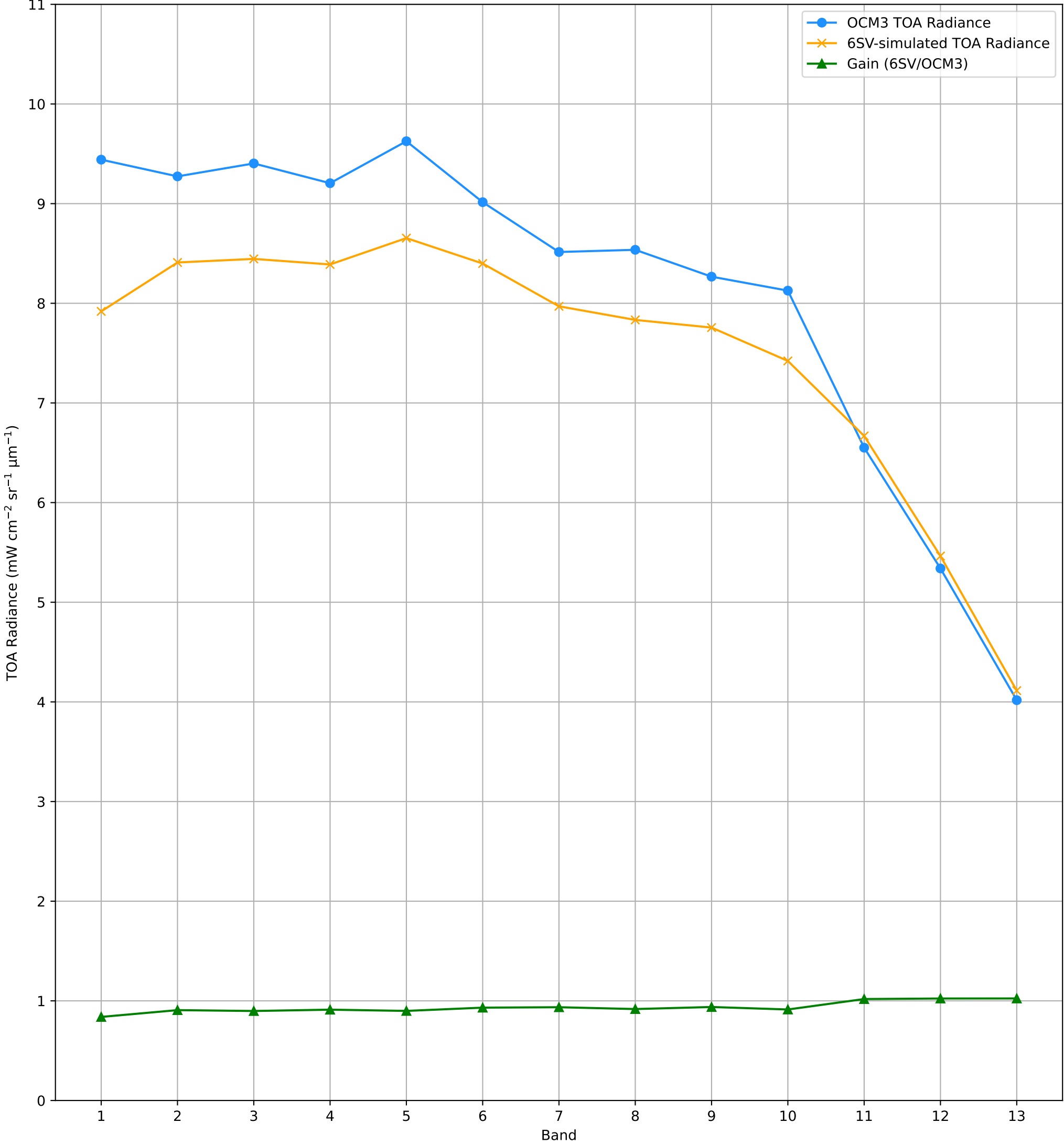
TOA Radiance (OCM3 vs. 6SV) over RVUS RadCalNet Site Lat: 38.497°, Lon: -115.69° - 12-DEC-2025 (STRIP_ID:16090)
