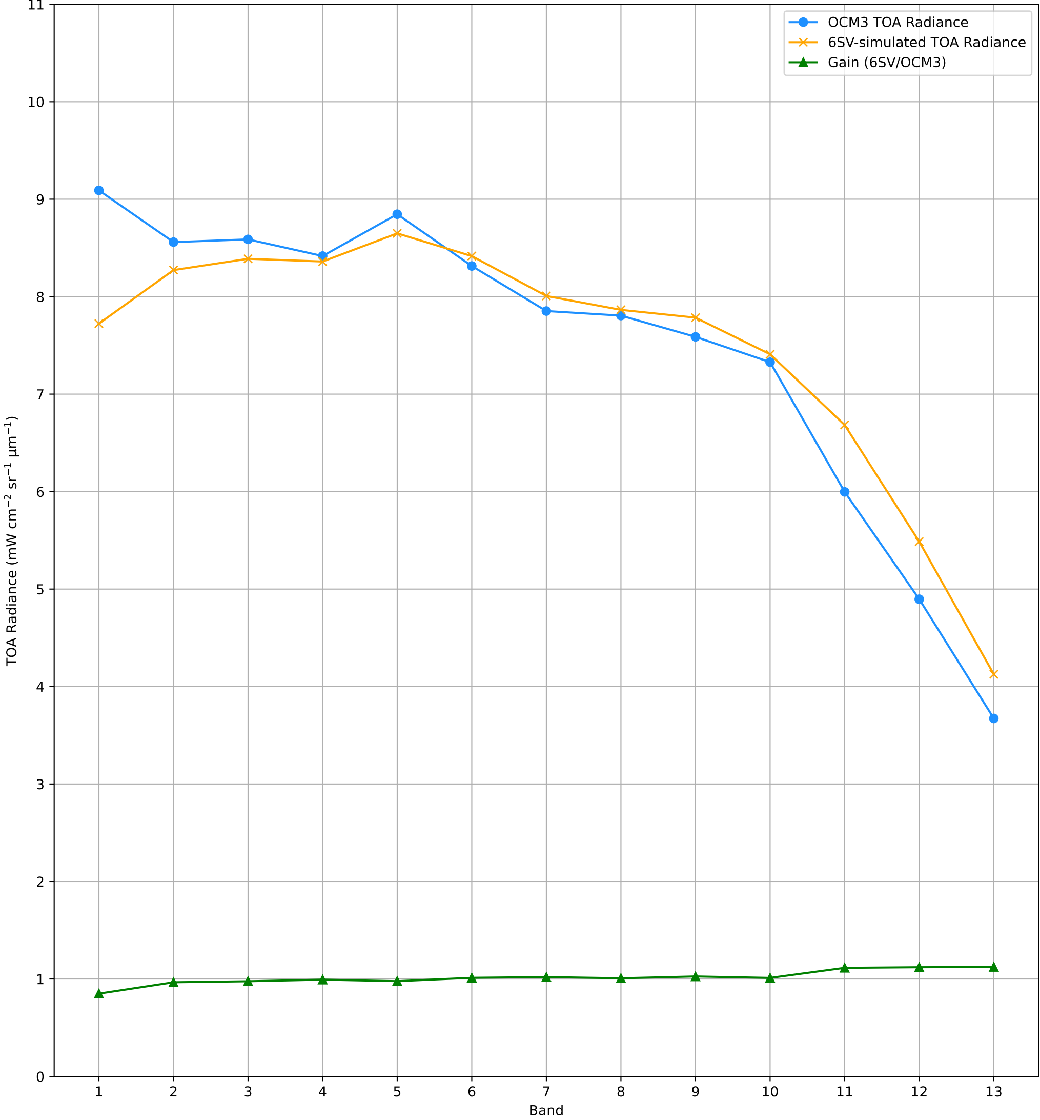
TOA Radiance (OCM3 vs. 6SV) over RVUS RadCalNet Site Lat: 38.497°, Lon: -115.69° - 16-DEC-2025 (STRIP_ID:16148)
