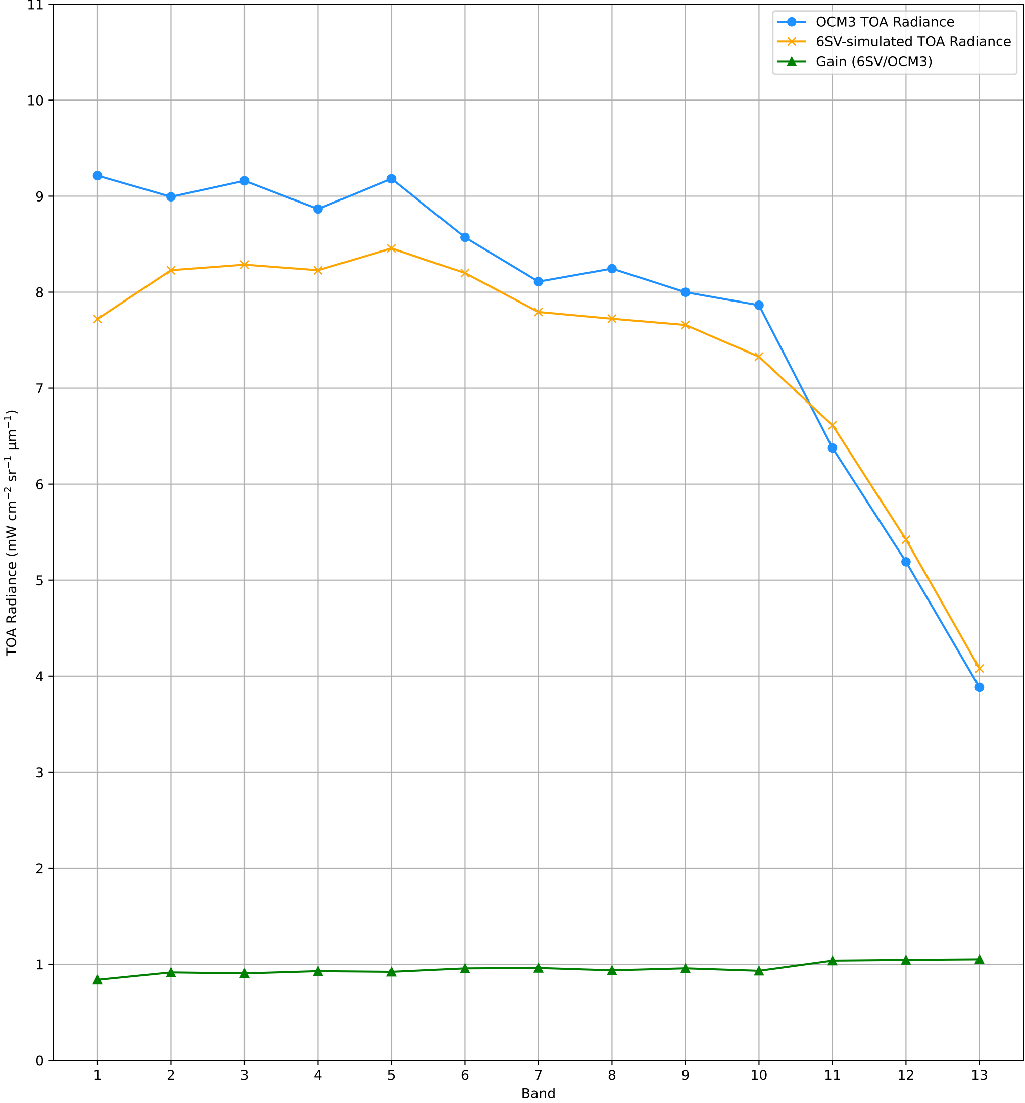
TOA Radiance (OCM3 vs. 6SV) over RVUS RadCalNet Site Lat: 38.497°, Lon: -115.69° - 27-DEC-2025 (STRIP_ID:16307)
