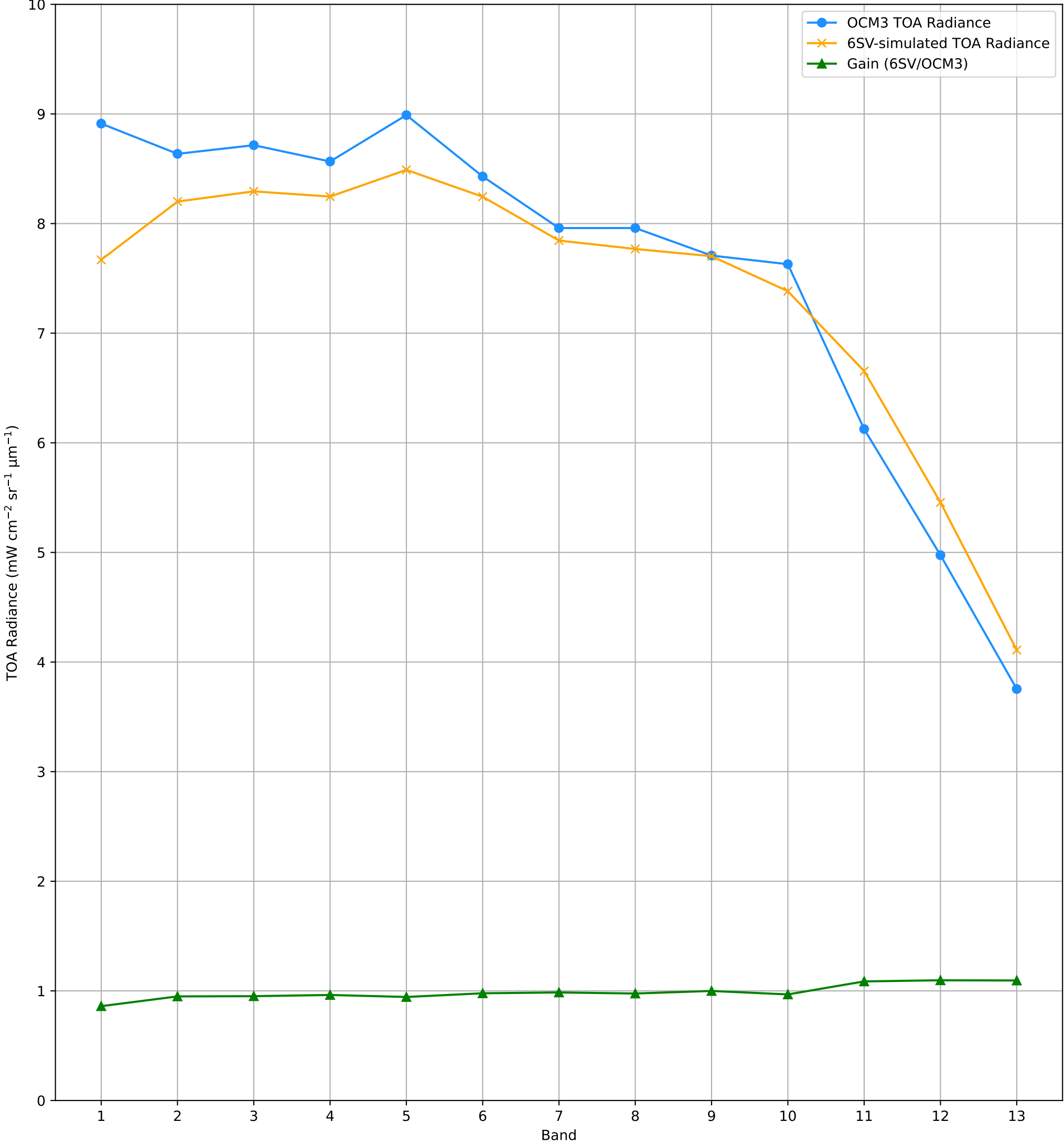
TOA Radiance (OCM3 vs. 6SV) over RVUS RadCalNet Site Lat: 38.497°, Lon: -115.69° - 29-DEC-2025 (STRIP_ID:16336)
