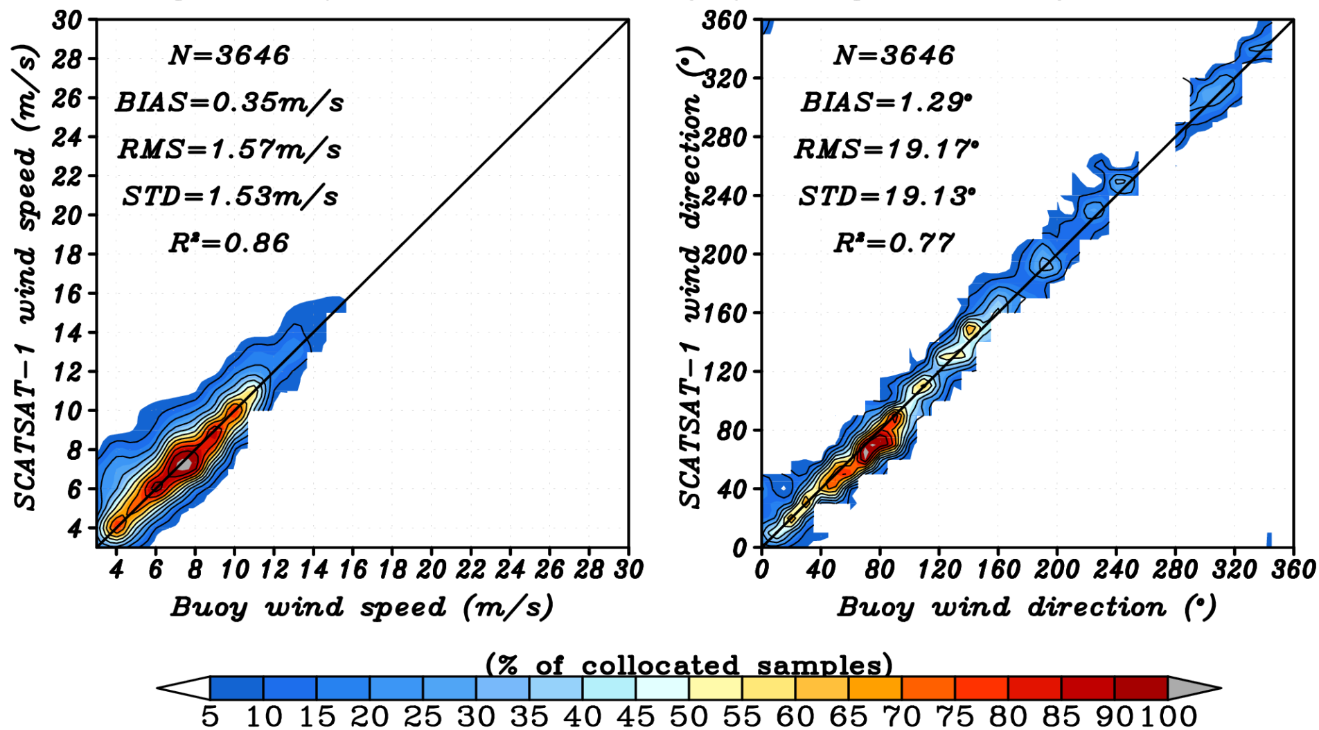
Comparison of SCATSAT-1 and Buoys for all passes over global oceans
