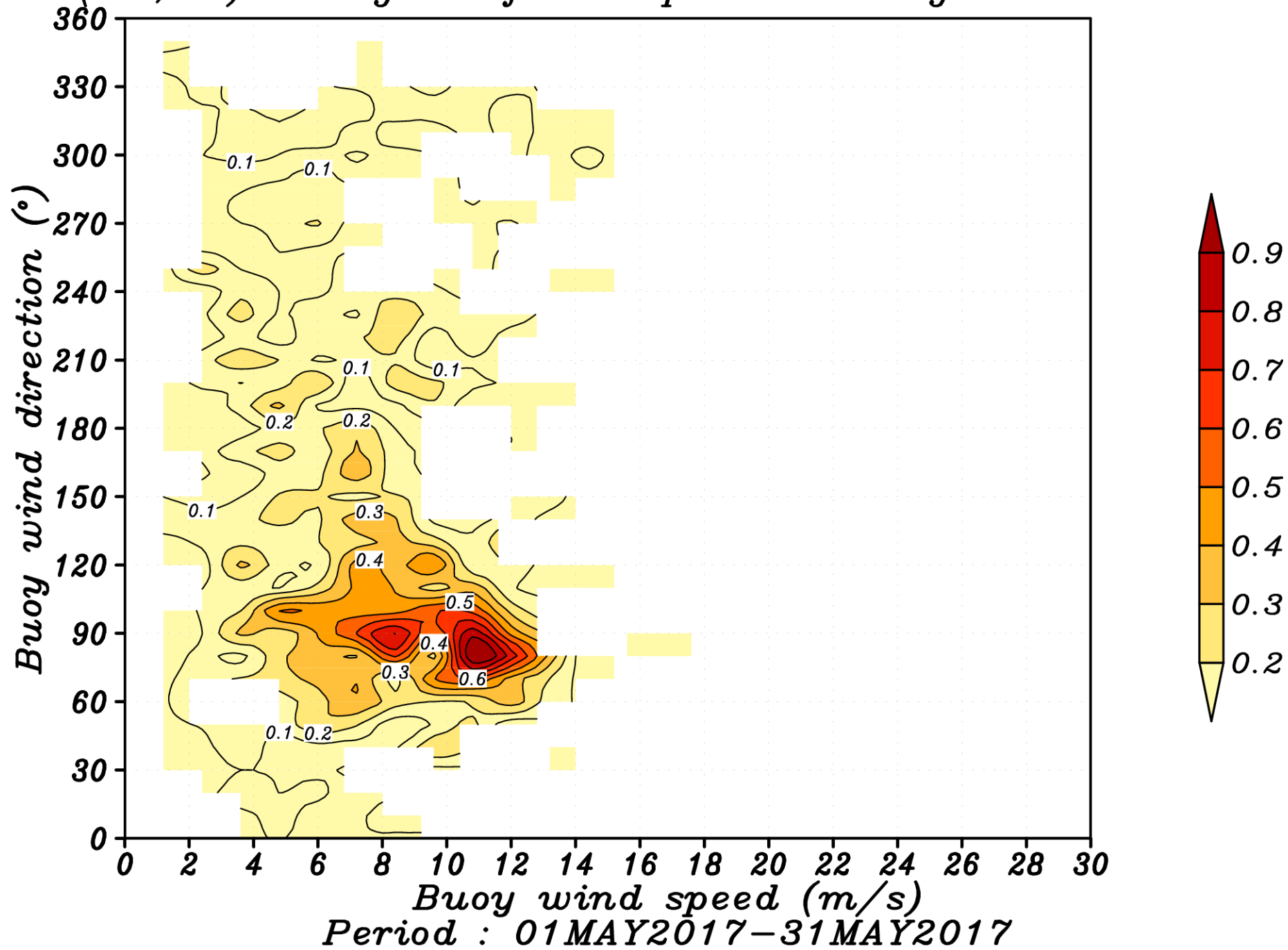
2D (WS,WD) Histogram for all passes over global oceans
