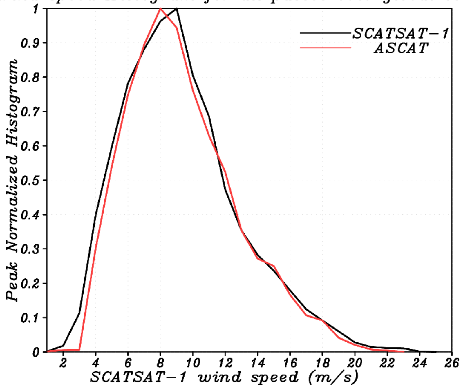
Wind speed Histogram for all passes over global oceans
