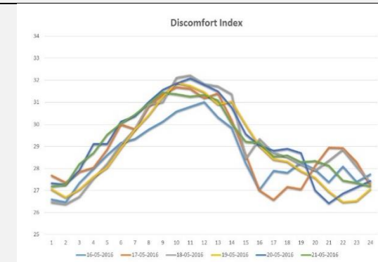
Diurnal evolution of Discomfort Index over Ahmedabad for different days of May 2016.
