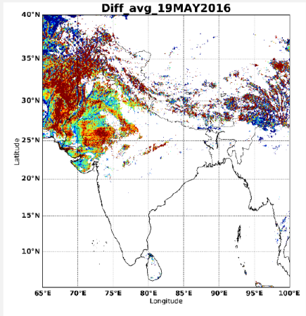
LST anomaly (°C) for 19 May 2016 at 1430 Hrs.
